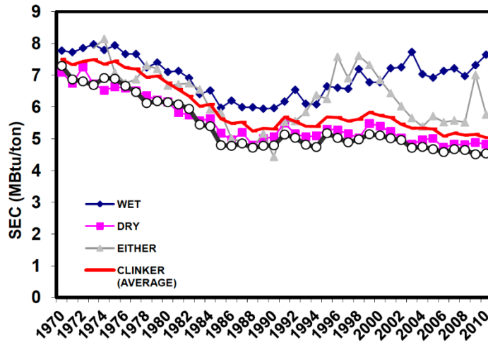
Worrell 2013 Figure 6. Primary energy intensity of U.S. cement and clinker production, 1970 to 2010 (MBtu/sh ton, HHV). This graph excludes use of wastes as kiln fuel between 1977 and 1992, as USGS did not collect this data before 1993.
